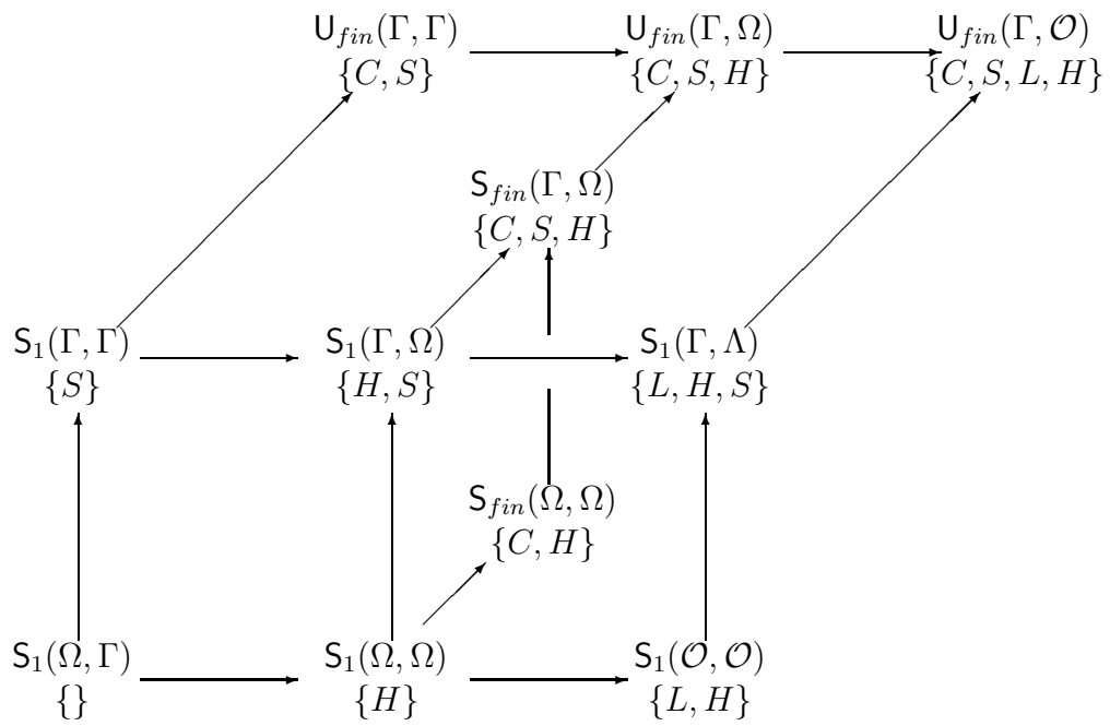
Figure 3: After removing equivalent classes
